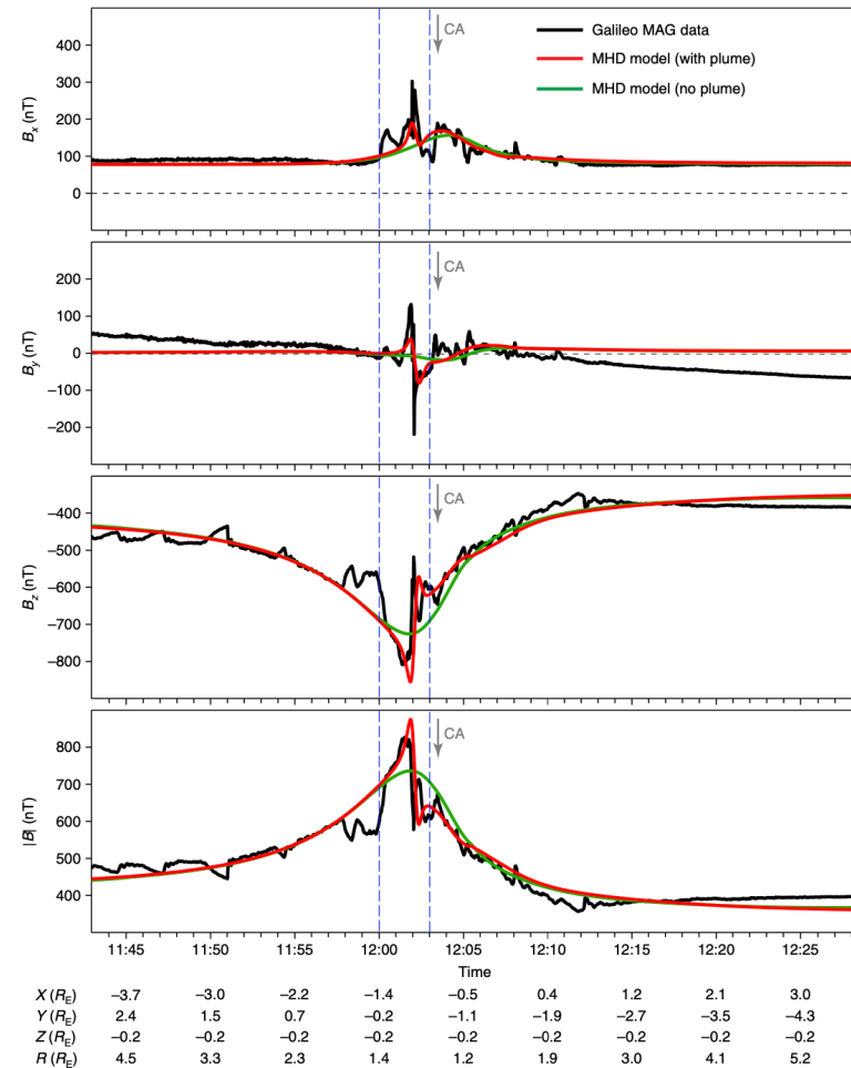
Fig. 1 | Galileo MAG data for the E12 flyby. Black lines show the MAG data. Green and red lines, respectively, show traces extracted from the MHD simulations without and with a plume included. Results are presented in EphiO coordinates, with x parallel to Europa's orbital velocity, y directed towards Jupiter and z completing the right-handed system. The interval of anomalous changes (~12:00 to 12:03 ut) is bounded by vertical dashed lines, and closest approach is marked by 'CA' and a grey arrow. In the range used for these measurements, the MAG sensor digitization step a was 0.25 nT. Between 11:55 and 12:05 ut, one or another of the 3 sensors saturated at the spacecraft rotation period. This required special processing, which increased the uncertainty to a level of a few nT. X, Y, Z and R given at the bottom of the figure indicate the spacecraft location and its radial distance from Europa's centre in units of R_E in EphiO coordinates.
