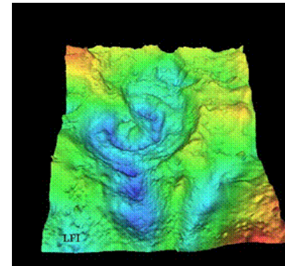
K-T event, \sim 65 million years ago (10 km, 10^8 megaton)
