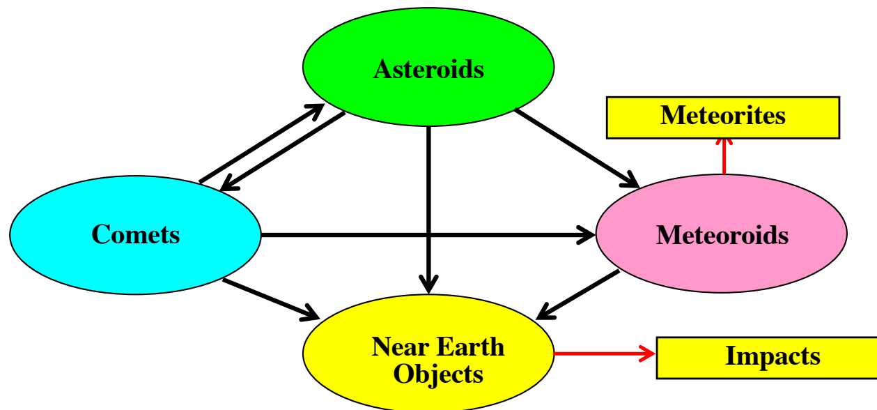
Minor bodies of the Solar System
