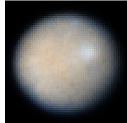
Ceres from DAWN
