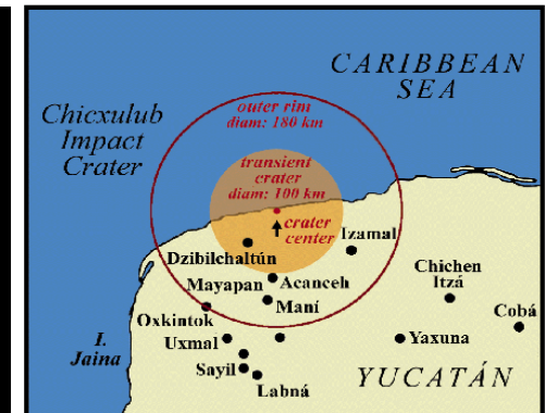
K-T event, \sim 65 million years ago (10 km, 10^8 megaton)
