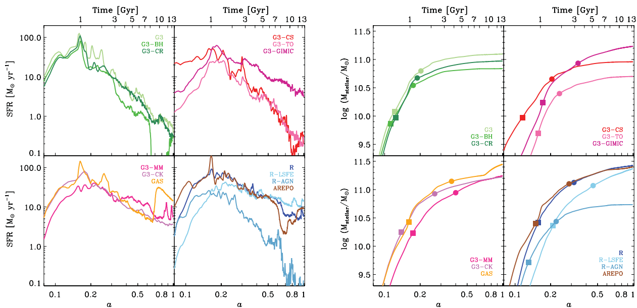
Figure 11. Distribution of stellar formation times (expressed in terms of the expansion factor, a ). Left- and right-hand panels show the same data, in differential and cumulative form, respectively. The simulations are grouped according to numerical technique, as in Fig. 5. The squares and circles indicate the time of formation of the first 10 and 50 per cent of the stars.
