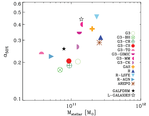
Figure 10. Median formation time of stars in the galaxy (expressed in terms of the expansion factor ( a_{50\text{ per cent}} )) as a function of total stellar mass at z = 0 . We also show the prediction of the semi-analytic models GALFORM (Cooper et al. 2010) and L-GALAXIES (Guo et al. 2011) for Aq-C.
