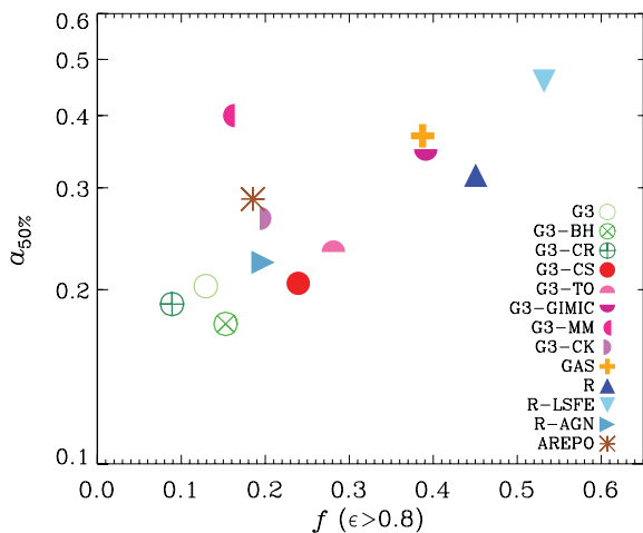
Figure 4. Median formation time of stars in the galaxy at z = 0 , expressed in terms of the expansion factor, a_{50\text{ per cent}} = 1/(1 + z_{50\text{ per cent}}) , as a function of the fraction of stars with circularity exceeding 0.8.
