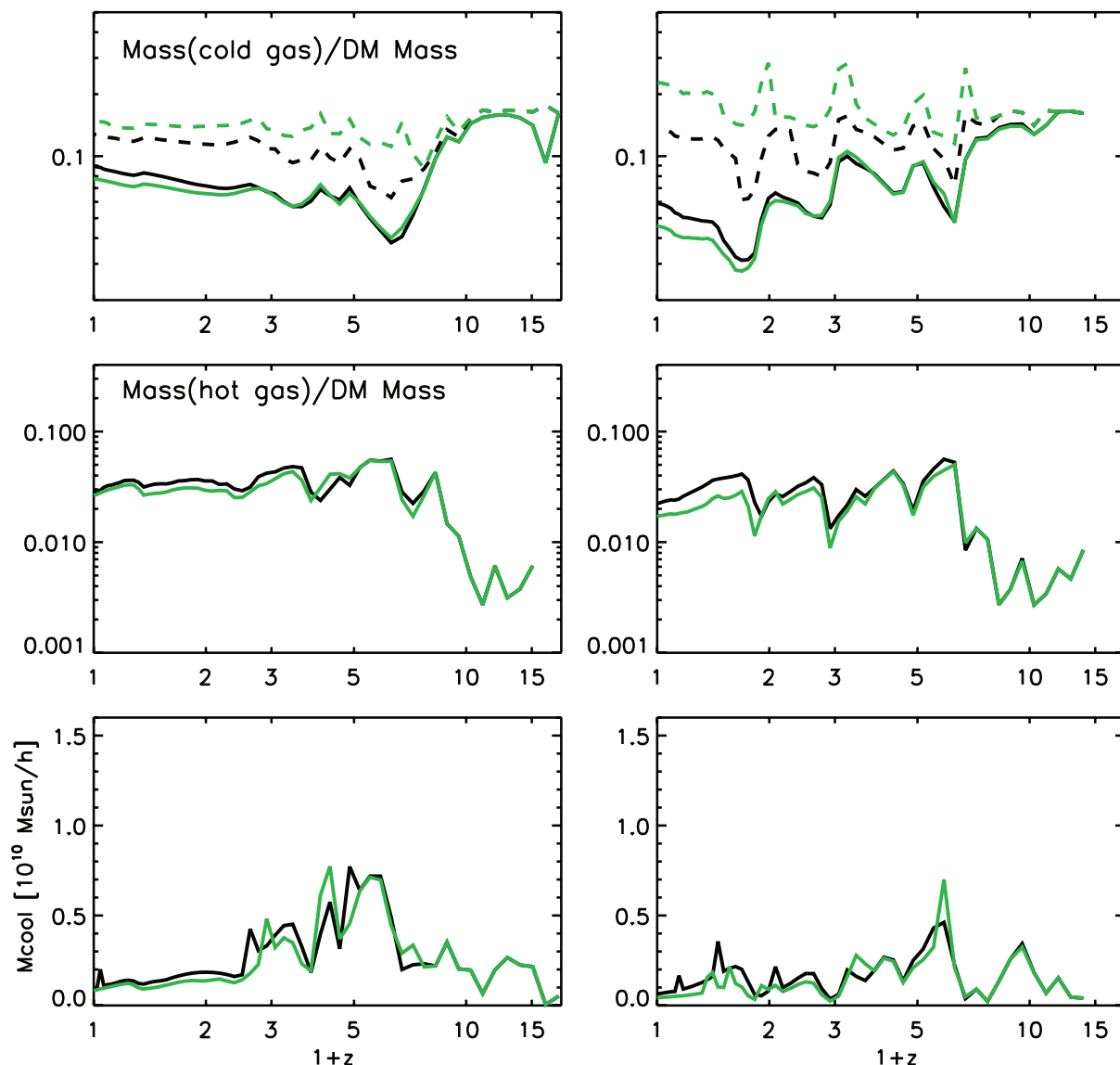
Figure 10. From top to bottom: cold gas fraction, hot gas fraction and gas cooling rate for the same MW-like haloes shown in Fig. 1. Solid and dashed lines in the top panels show results for the t_{\text{mrg}} = \infty and t_{\text{mrg}} = 0 runs, respectively. Black and green lines correspond to subhalo- and FOF-based merger trees, respectively.
