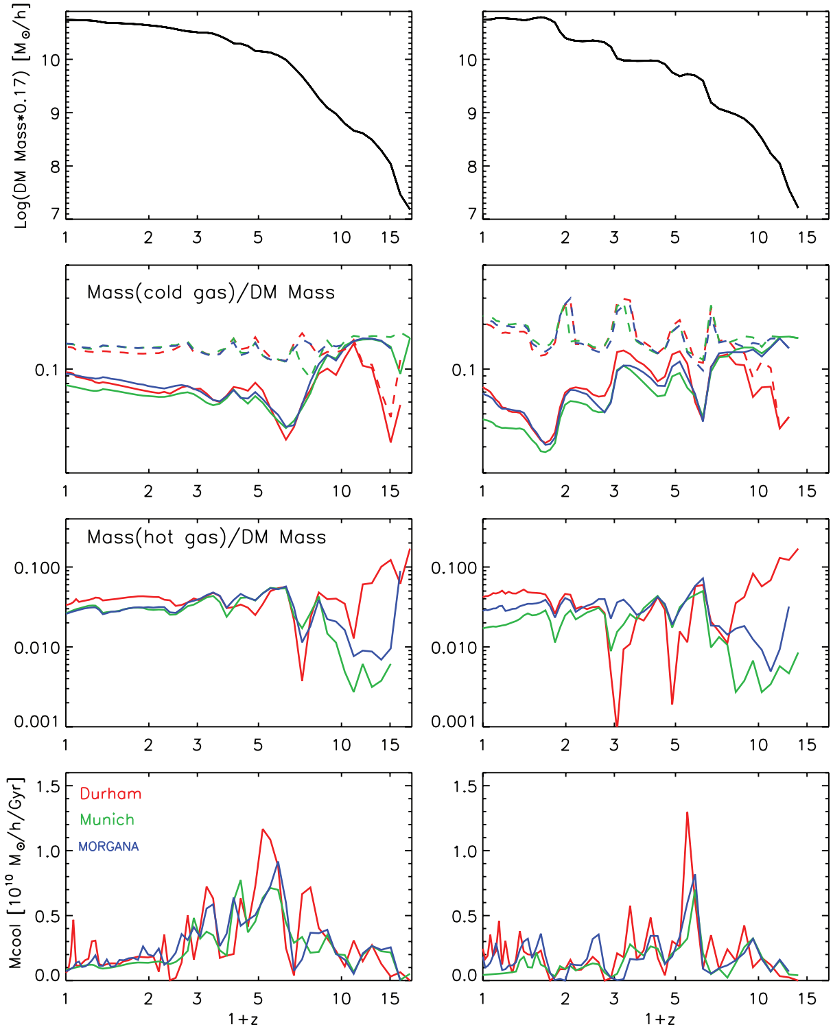
Figure 1. From top to bottom: dark matter, cold gas, hot gas and gas cooling rate for two MW-like haloes. Only quantities associated with the central galaxy and its main progenitors are plotted. Red lines show results from the Durham model, green lines show results from the Munich model and blue lines are for MORGANA. Solid and dashed lines in the second panels from the top show results for the t_{\text{mrg}} = \infty and t_{\text{mrg}} = 0 runs, respectively. The haloes shown in this figure provide two representative examples for a halo with a rather quiet mass accretion history (left-hand panels) and a halo with a larger number of massive mergers (right-hand panels).
