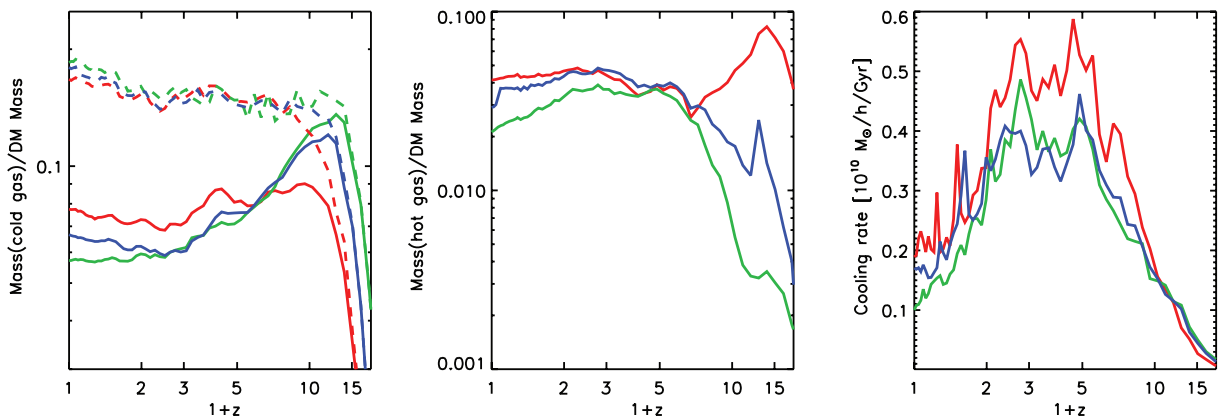
Figure 2. From left- to right-hand panels: cold gas, hot gas and gas cooling between two subsequent snapshots. Each line shows the average computed over 100 MW-like haloes. Solid and dashed lines in the left-hand panels show results for the t_{\text{mrg}} = \infty and t_{\text{mrg}} = 0 runs, respectively. Colour coding is as in Fig. 1.
