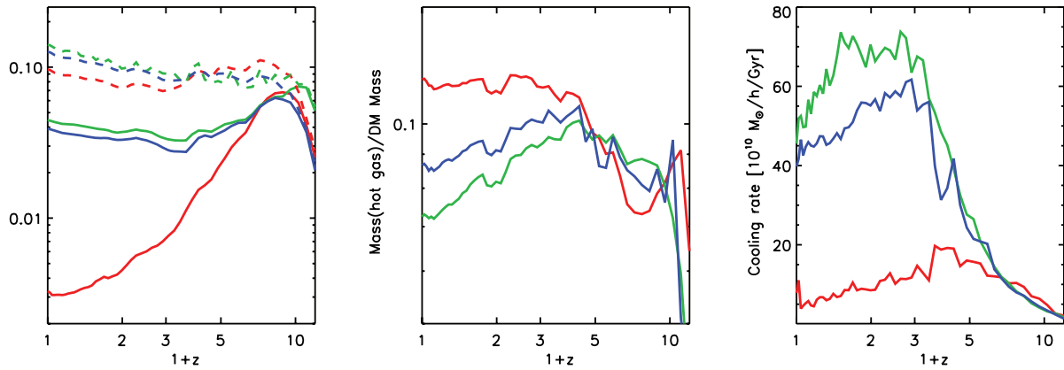
Figure 5. Same as in Fig. 2, but for the SCUBA sample.
