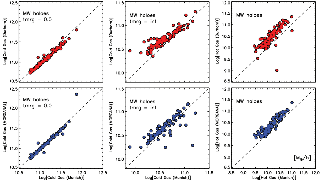
Figure 3. Cold gas for the t_{\text{mrg}} = 0 case (left-hand panels), cold gas for the t_{\text{mrg}} = \infty case (middle panels) and hot gas (right-hand panels) associated with the central galaxy for the MW sample. Top panels show results obtained by the Durham code against those from the Munich model. Bottom panels show results by the MORGANA code against those from the Munich model. The dashed line is the one-to-one relation and is plotted to guide the eye.
