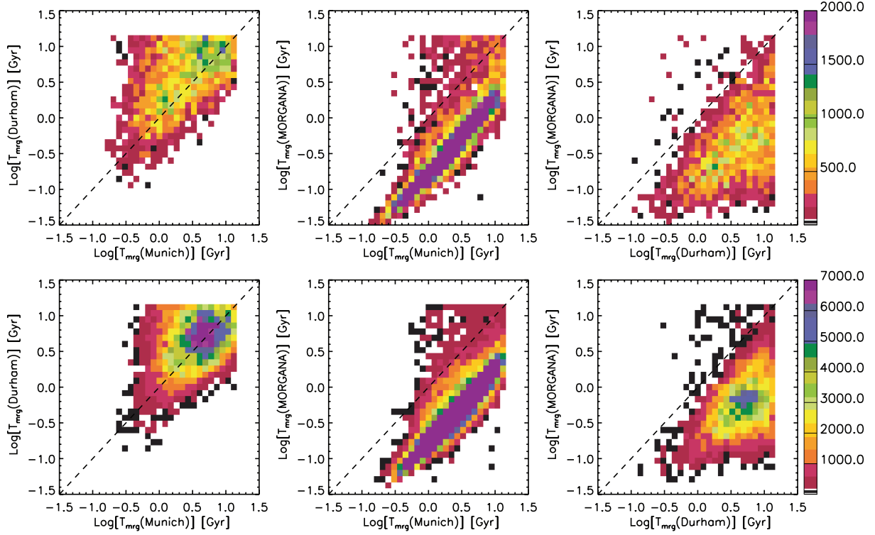
Figure 12. Distributions of merging times in the three models used in this paper. Top panels are for MW haloes while bottom panels are for the SCUBA haloes. Maps have been computed using only satellite galaxies present in both models and with merger time smaller than the Hubble time.
