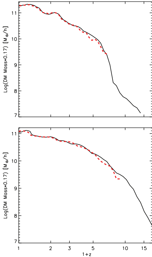
Figure 7. Mass accretion history of two of the haloes from the MW-like sample used in this paper, at two different resolution levels. Solid lines show the histories constructed using the MS-II simulation, while dashed lines show the corresponding histories from the mini-MSII.
