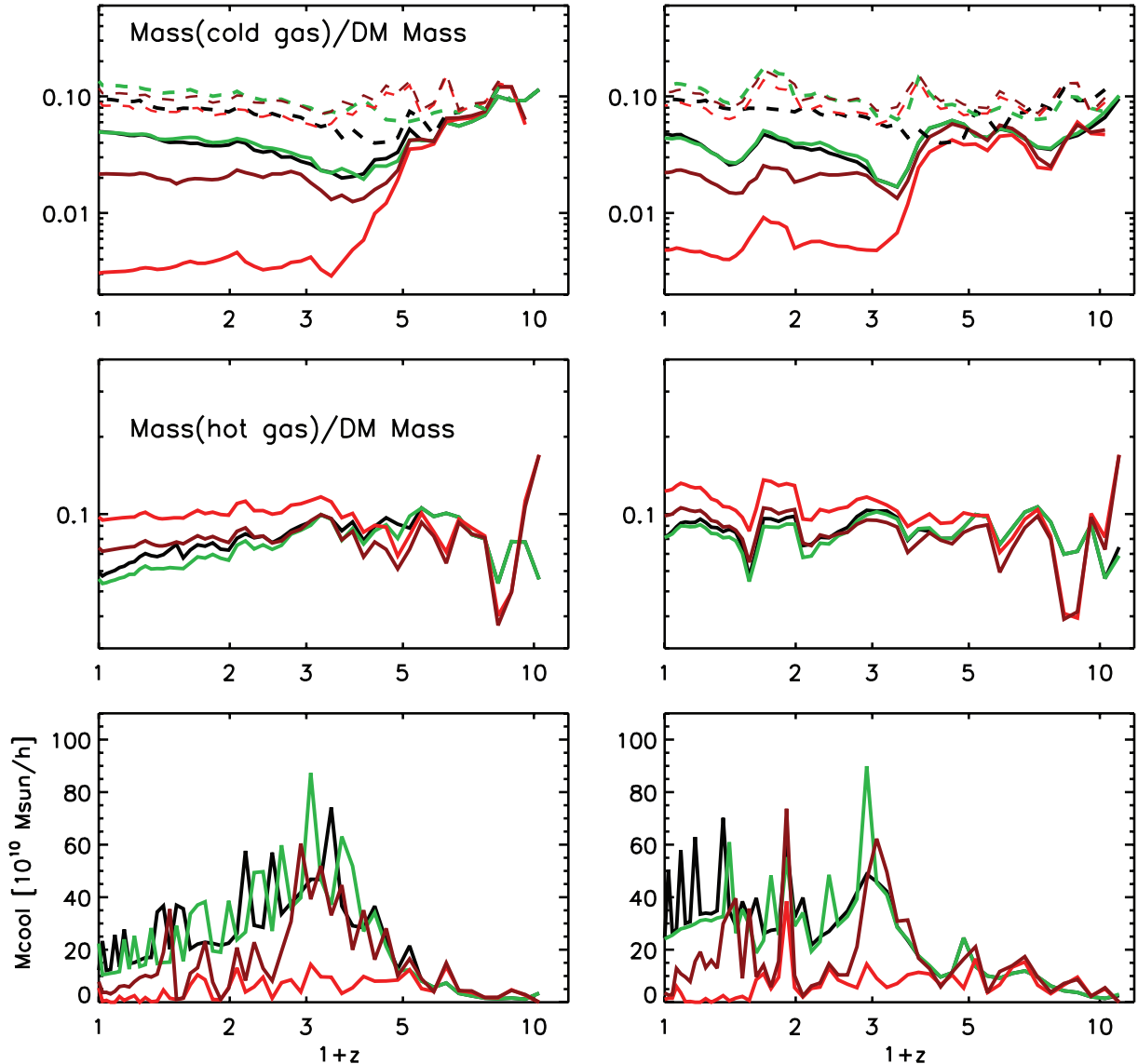
Figure 11. From top to bottom: cold gas fraction, hot gas fraction and gas cooling rate for the same SCUBA haloes shown in Fig. 4. Solid and dashed lines in the top panels show results for t_{\text{mrg}} = \infty and t_{\text{mrg}} = 0 , respectively. Black and green lines correspond to subhalo- and FOF-based merger trees, while red lines correspond to the outputs from the Durham model, with darker lines showing results obtained assuming an isothermal profile for the hot gas.
