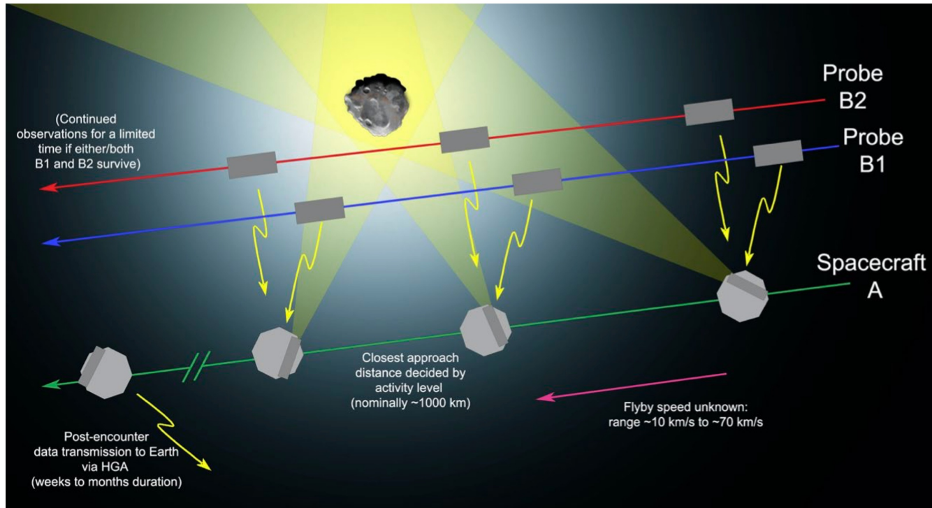
Figure 1: Sketch of the Comet Interceptor flyby, not to scale. Spacecraft A will pass furthest from the nucleus, with Probes B1 and B2 passing closer. Both probes will relay their data in real time to be stored on Spacecraft A.
