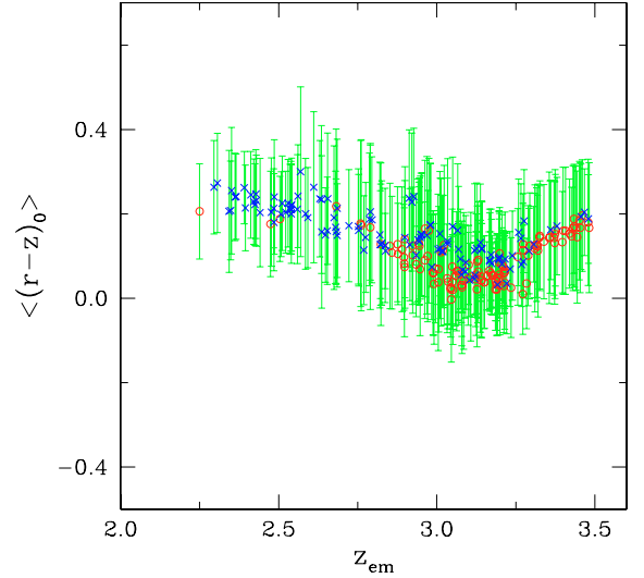
Fig. 2. Mean color \langle(r-z)_0\rangle of the QSOs control samples used to estimate the unreddened colors of the DLA-QSOs. The mean color is plotted versus the QSO redshift, z_c . Bright ( r < 19.1 mag) and faint ( r \geq 19.1 mag) QSOs are plotted with blue crosses and red circles, respectively.
