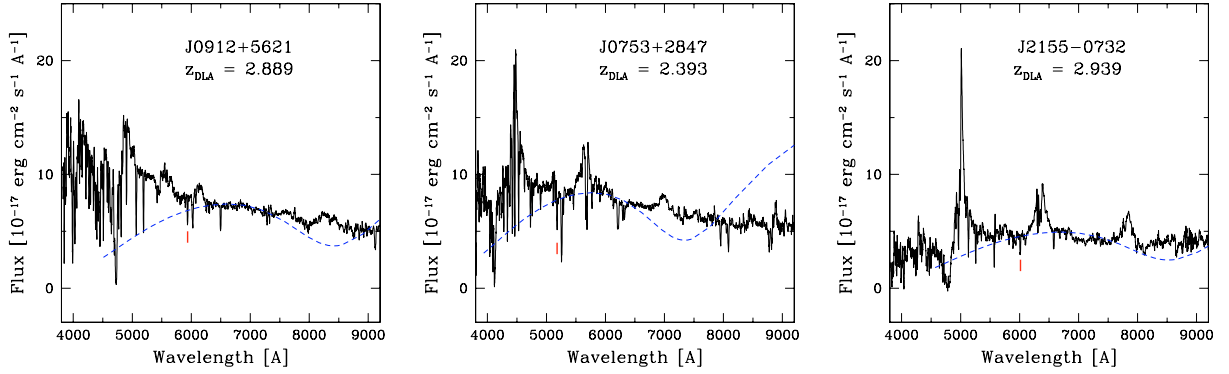
Fig. 8. Quasars of the absorption sample with color deviations \Delta(g - z) > 0.4 mag and strong Si II absorptions at z_{\text{SiII}} = z_{\text{DLA}} . Dashed line: profile of the 2175 Å extinction bump plotted in a scale 10^{-\xi[\lambda/(1+z_{\text{DLA}})]} (see Vladilo et al. 2006).
