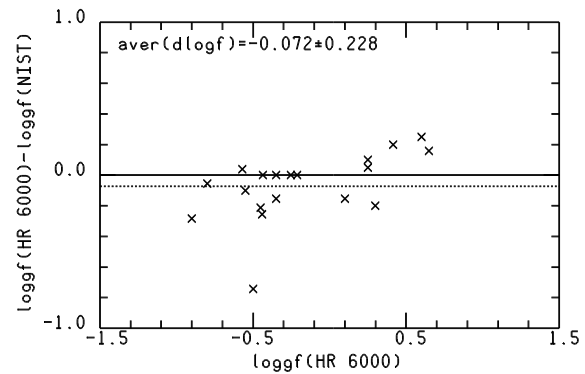
Fig. 1. Comparison of astrophysical \log gf -values of Xe II derived from HR 6000 with the \log gf -values of the NIST critical compilation.
