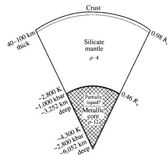
Model of Venus internal structure Fegley (2005)
